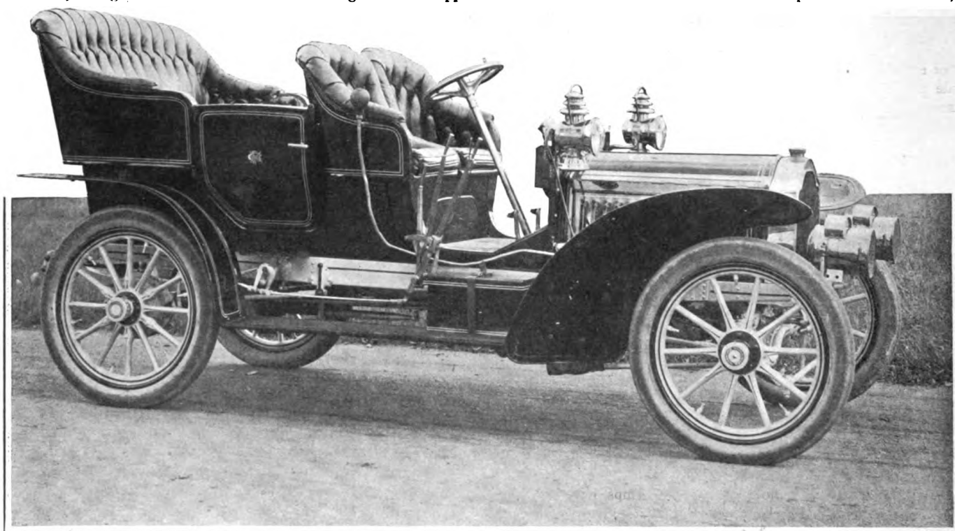
NEW 1905 MODEL N PACKARD 22-28 HORSEPOWER TOURING CAR, WITH SIDE ENTRANCE TO THE REAR SEAT.
